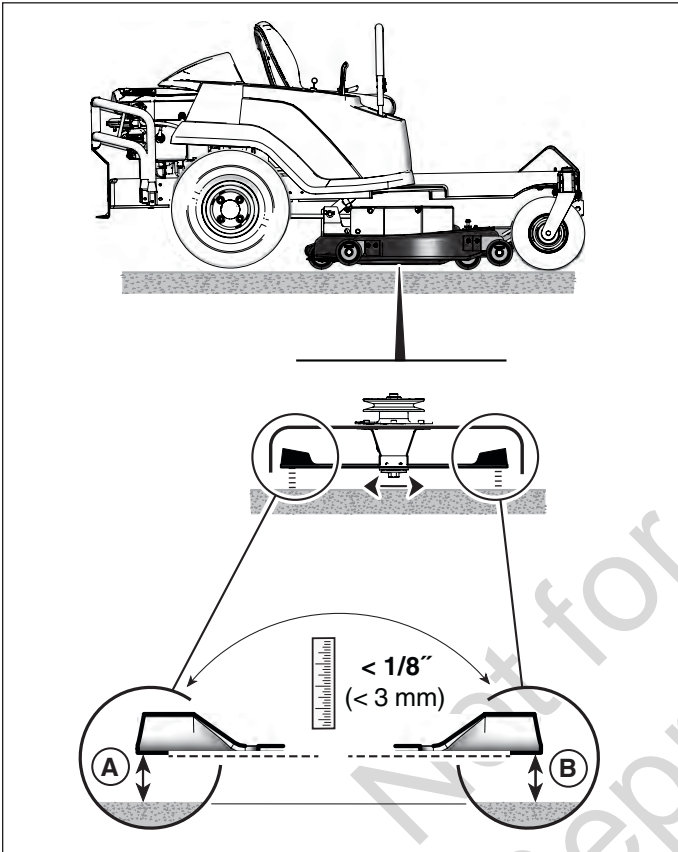
Figure 25. Mower Deck Level Check (Front-to-Back)
